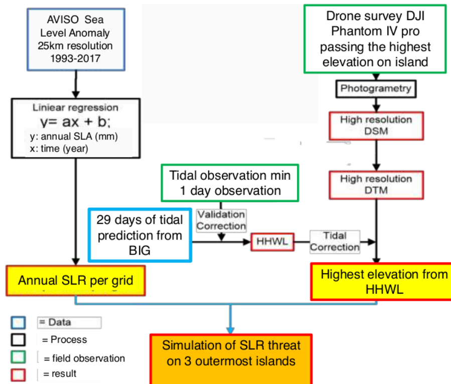
Fig. 2: Research Flowchart
