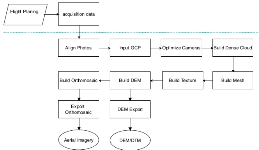
Fig. 3: Flowchart of photogrammetry method
