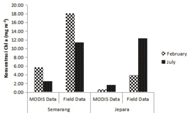
7 Figure 7. The average chlorophyll a in AQUA MODIS and the field observation in 2019
