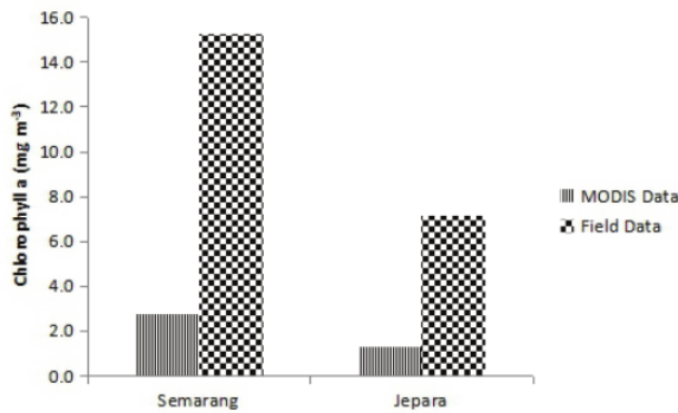
7 Figure 6. The average chlorophyll a in AQUA MODIS (2015–2019) and the field observation (2017–2019)
