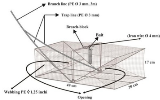
Figure 1 Construction of box fold trap
