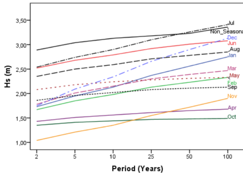
Figure 4. Non seasonal and monthly(seasonal) Return value.
