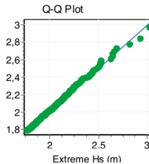
Figure 2. QQ plot for non-seasonal GPD
