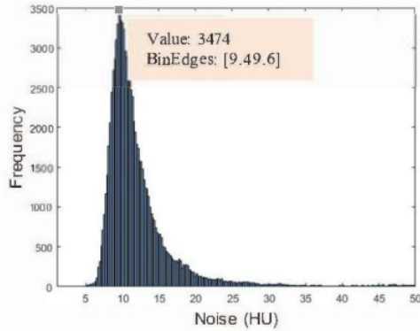
Figure 4. Noise Histogram
