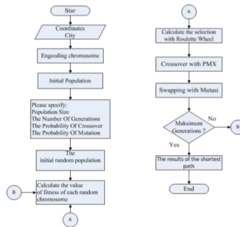
Fig.2 Genetic algorithm flowchart
