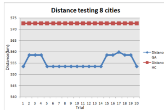
Fig. 4 Distance testing 8 cities
