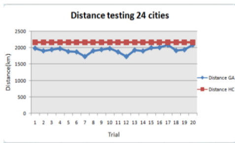
Fig. 6 Distance testing 24 cities
