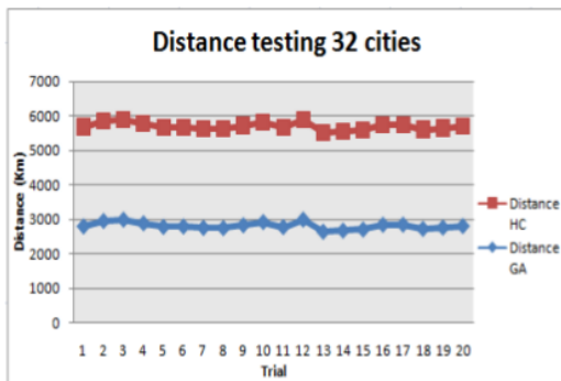
Fig. 7 Distance testing 32 cities
