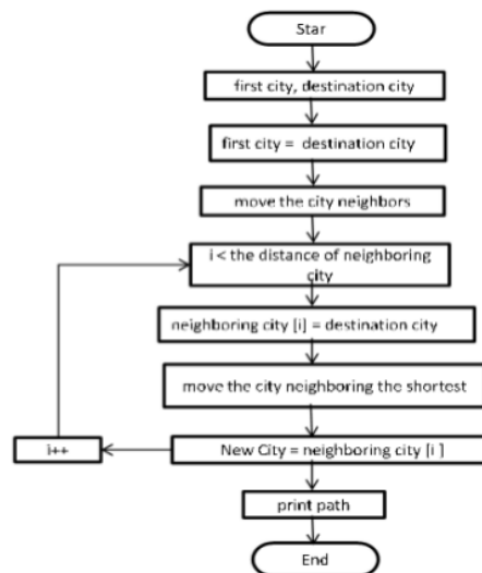
Fig. 3 Hill Climbing flowchart
