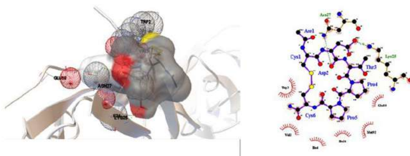
Figure 4. The interaction between cyclic ADTC6 peptide code S4 and the EC1-EC2 domain of E-cadherin with used (a) Autodock program, and (b) Ligplus program.
