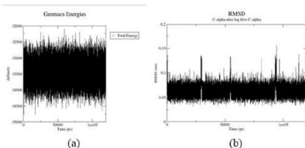
Figure 3. (a) The total energy graph of cyclic ADTC6 120 ns, (b) The RMSD profile of cyclic ADTC6.
