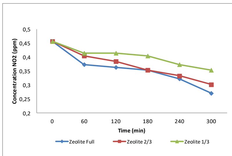
Figure 2. Decrease in \text{NO}_2 concentration with different amounts of zeolite
