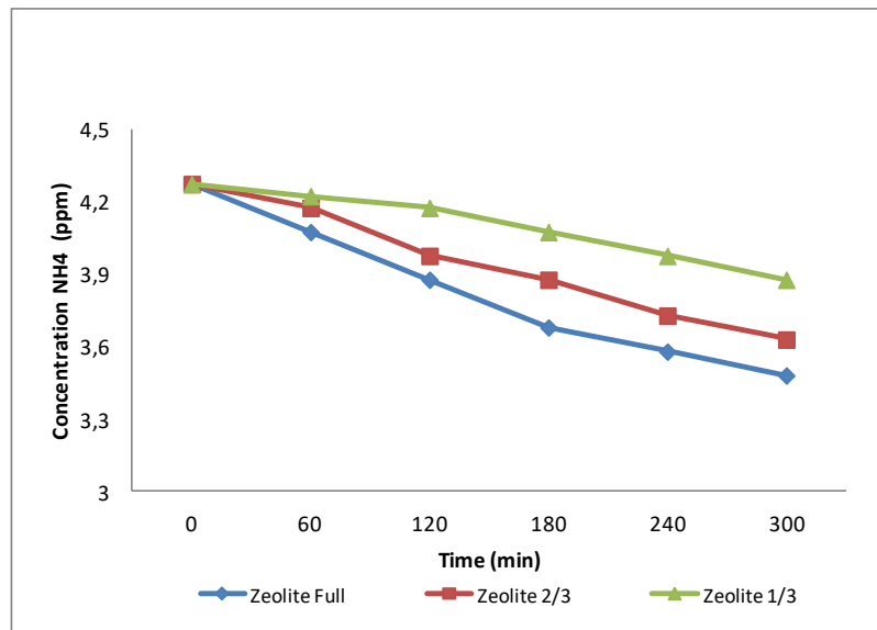
Figure 1. Decrease in \text{NH}_4 concentration with different amounts of zeolite
