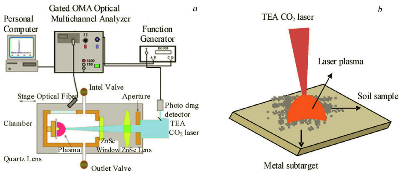
Fig. 1. Basic setup (a), and illustration of the sample holder employed in this study (b).
