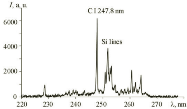
Fig. 2. C spectrum obtained from the garden soil.
