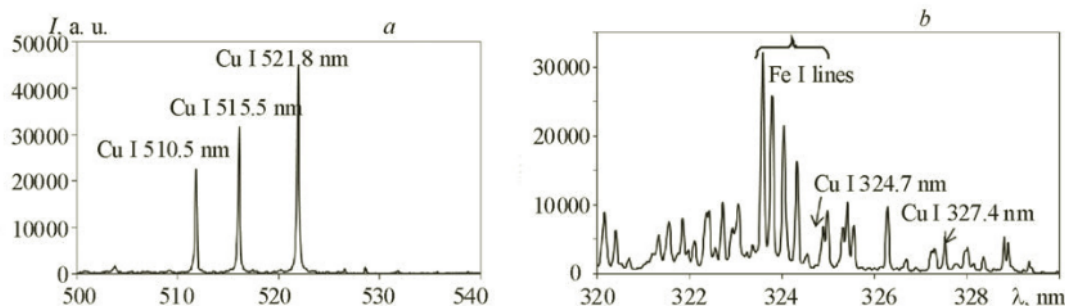
Fig. 4. Emission spectrum of Cu obtained (a) from the powdered CuSO 4 using mesh assisted gas plasma method, and (b) from the standard soil containing 50 mg/kg Cu.
