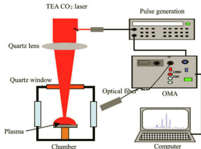
1 Fig. 1. Experimental setup used in this work.
