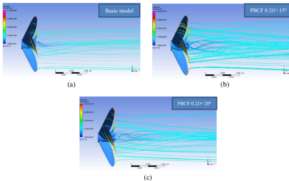
Figure 6. Streamline of propeller before and after installation of PBCF
