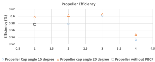
Figure 5. Comparison of propeller Efficiency before and after installation PBCF
