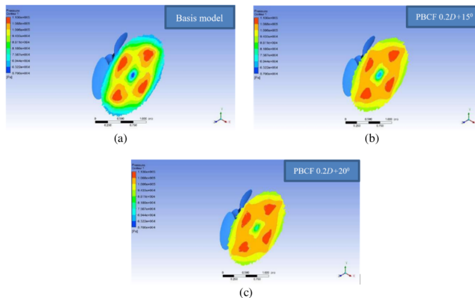
Figure 7. Pressure contour before PBCF with and after installation PBCF located in the rear propeller
