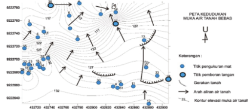
Fig. 3. Unconfined flow networks at research location.
