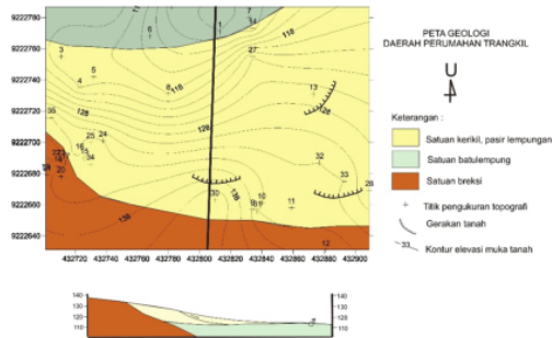
Fig. 2. Technical geological map of Trangkil settlement.
