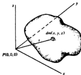
Gambar 3 Potensial Massa Tiga Dimensi [7]
