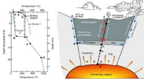
Gambar 1. Model Sistem Geotermal [4]
