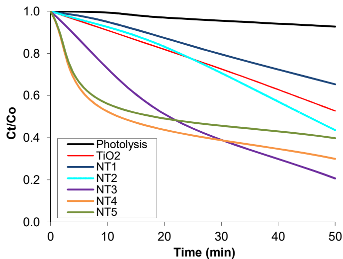
Figure 3. Photocatalytic degradation of MB by as-prepared samples under solar radiation.
