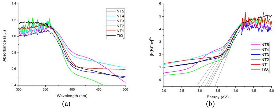
Figure 2. (a) Absorption spectra of all prepared samples, and (b) Diffuse reflectance UV-vis spectra of all prepared samples.
