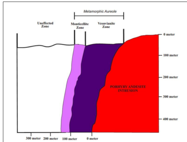
Figure 14. The vertical cross section of contact metamorphism effect zonation at Selo Gajah Hill, Jari Village, Gondang Sub district, Bojonegoro
