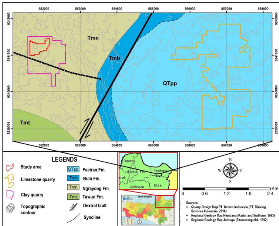
Figure 1. Regional geology map.
