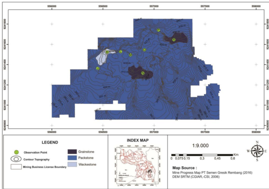
Figure 2. Geological map of research area.
