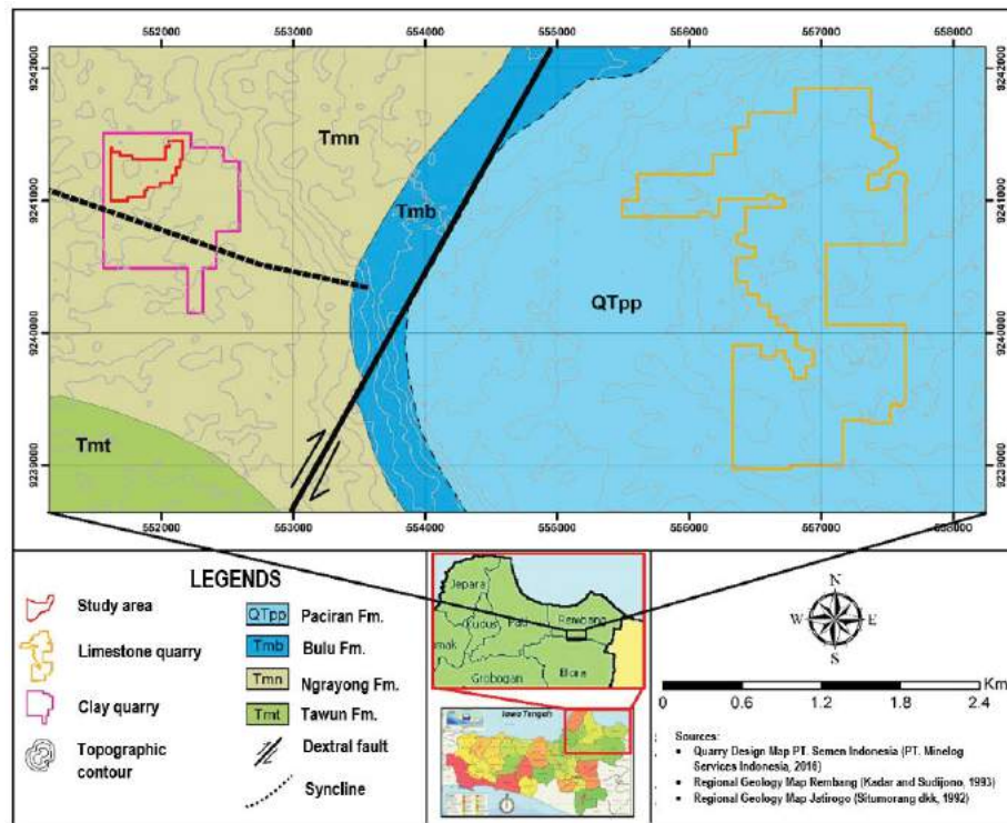
FIGURE 2. Regional geology map
