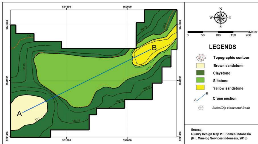
FIGURE 3. Geological map of research area
