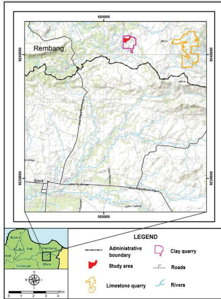
FIGURE 1. Research area location
