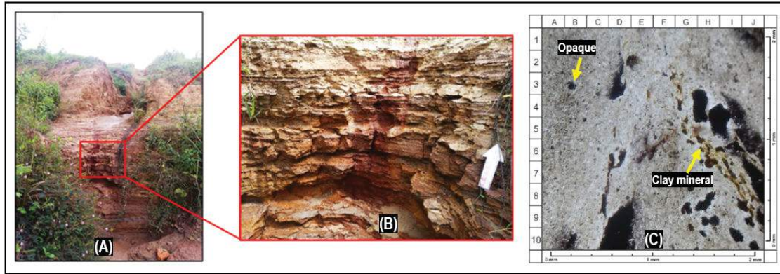
FIGURE 6. Outcrop of claystone (A, B) and its petrographic thin section (C)
