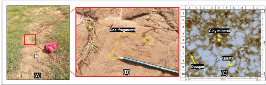
FIGURE 7. Outcrop of brown sandstone with coal fragments (A, B) and its petrographic thin section (C)
