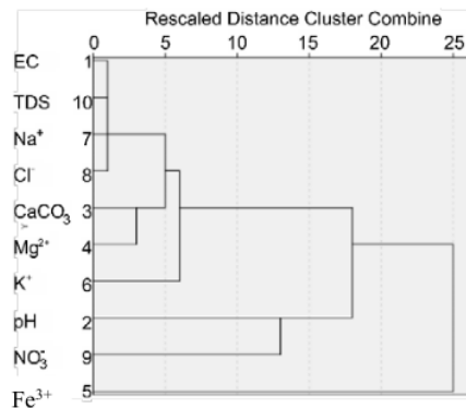
Fig. 5 Cluster analysis
