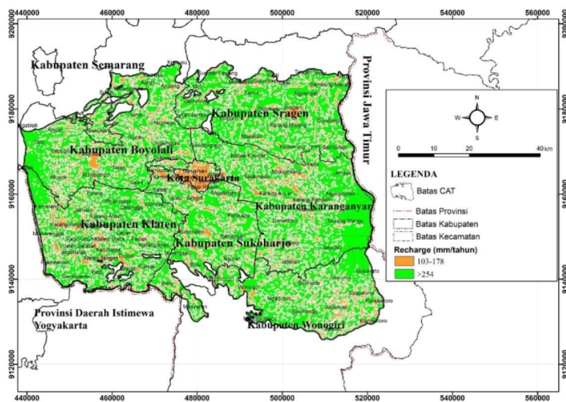
Gambar 5. Peta Recharge
