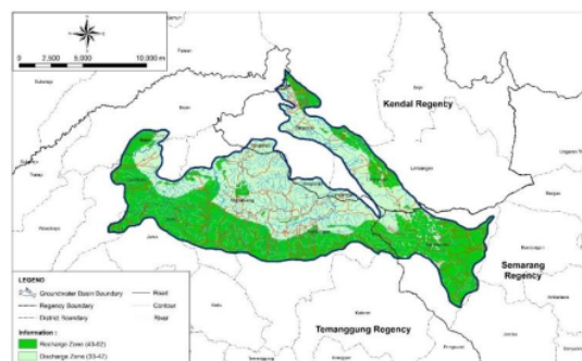
Figure 7. The recharge zone of Sumowono groundwater basin.
