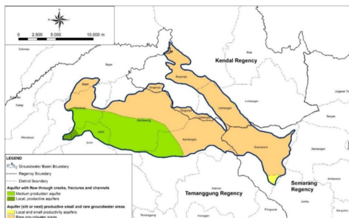
Figure 3. Regional hydrogeological map of Sumowono groundwater basin.
