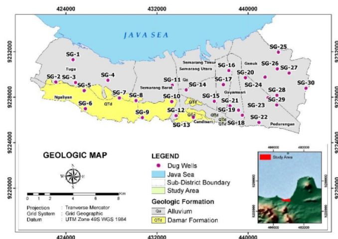
Figure 1. The study area and its geologic setting
