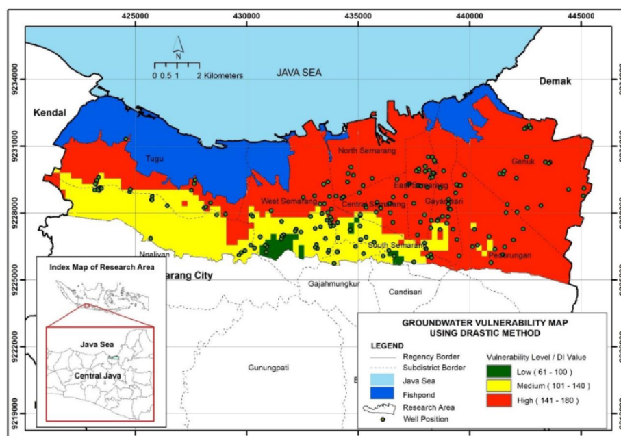
Figure 3. Groundwater vulnerability map using DRASTIC method.
