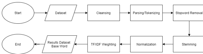
Figure 1. Flow diagram sentiment analysis process
