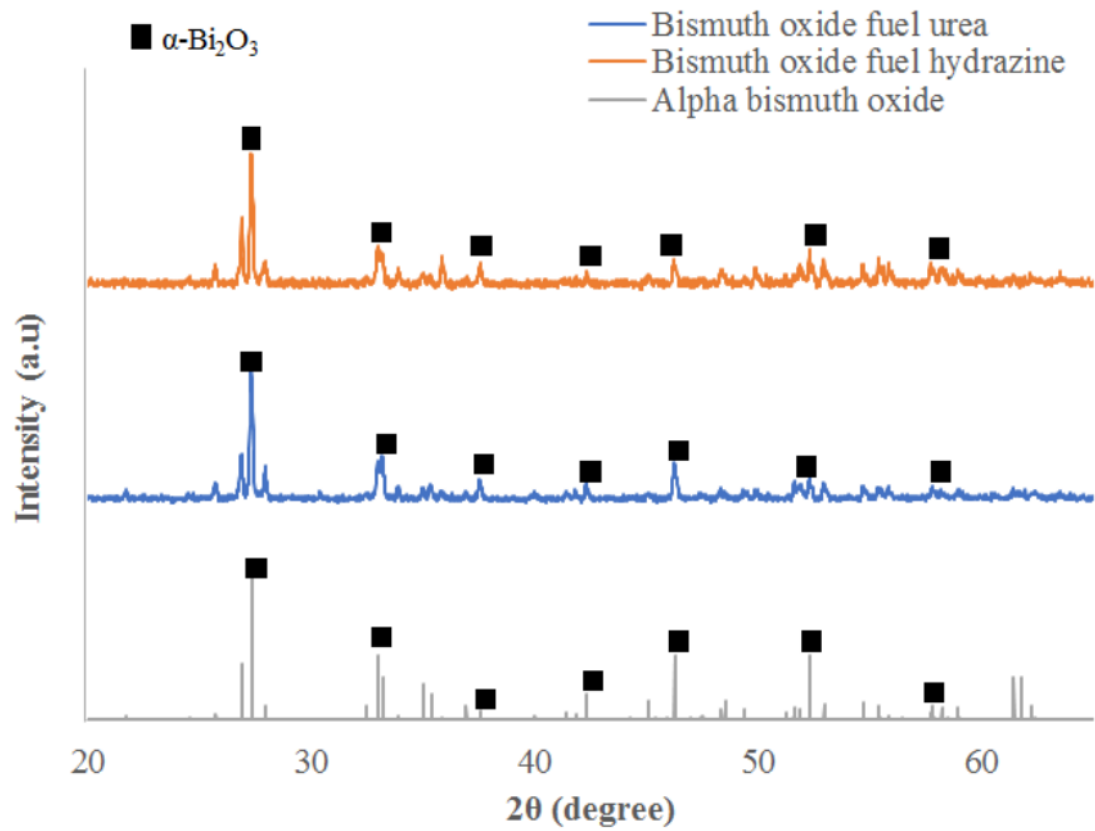
Figure 4. XRD Diffractograms of synthesized bismuth oxide
