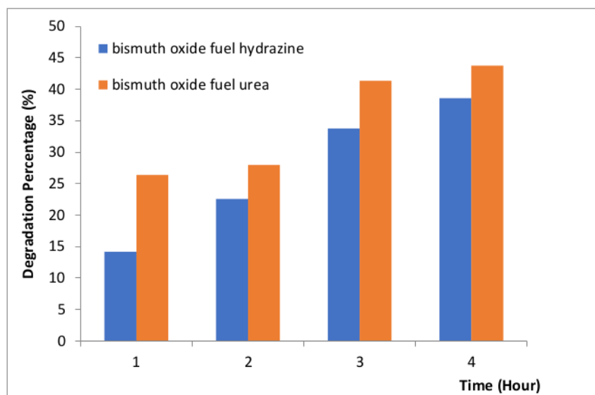
Figure 7. Photocatalytic time effect on the percentage of Rhodamine B concentration degraded by \text{Bi}_2\text{O}_3 synthesized by urea (BO1) and hydrazine (BO2)
