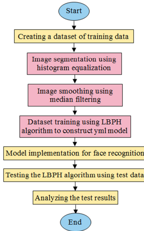
Fig. 1 Block diagram of research procedure
