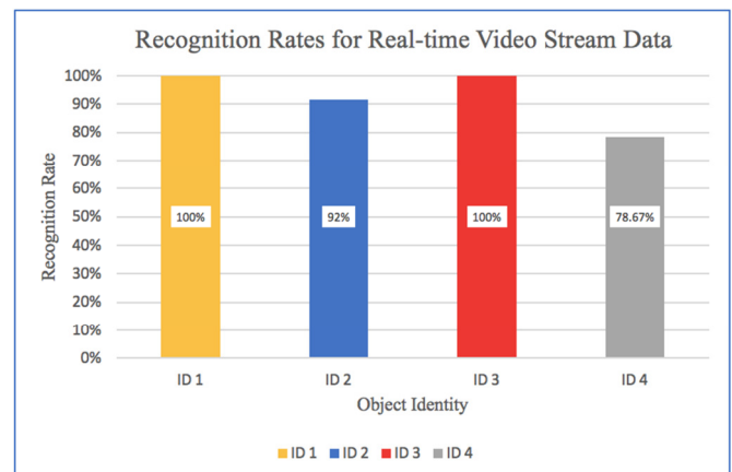
Fig. 13 Number of successful recognitions using real-time video stream data
