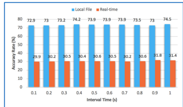
Fig. 9 Accuracy rate for two faces in one frame
