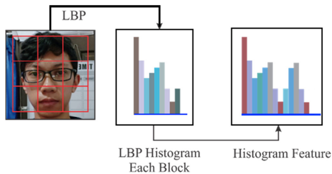
(b) LBP process for each histogram
