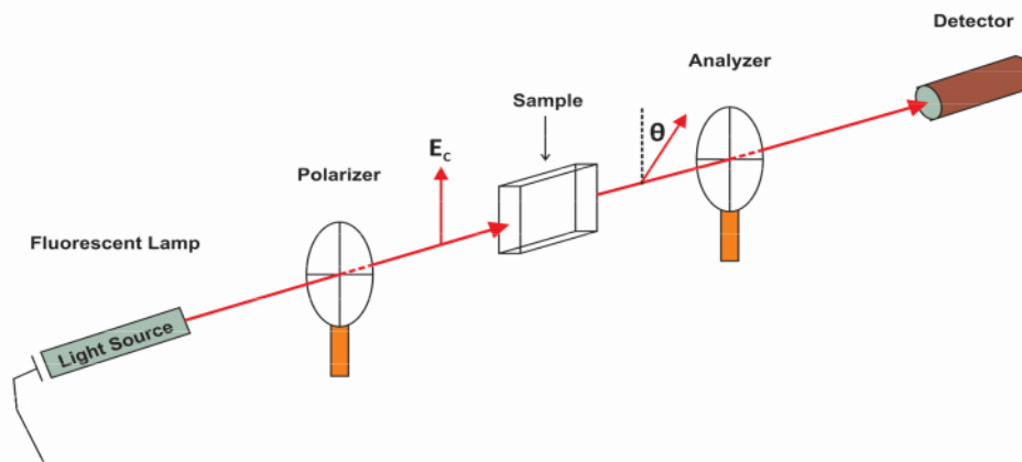
Fig.-1: Experimental setup of the electro-optical method
