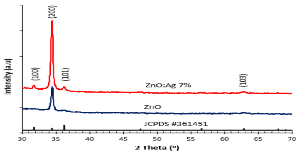
Fig.-2: Thin film XRD-spectra of ZnO and ZnO:Ag.
