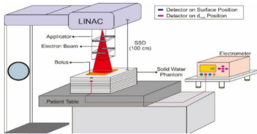
Figure 3: Schematic data collection using bolus
