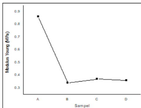
Figure 7: Modulus young values of each sample
