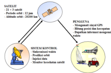
Figure 1. Segment of GNSS
