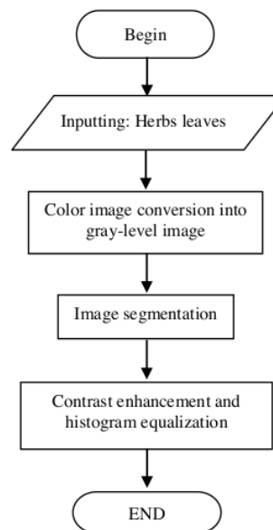
Fig. 1 Preprocessing flowchart
