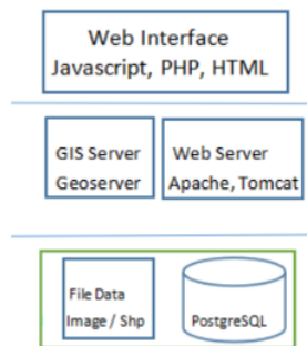
Figure 1 VGI WebGIS Architecture System
