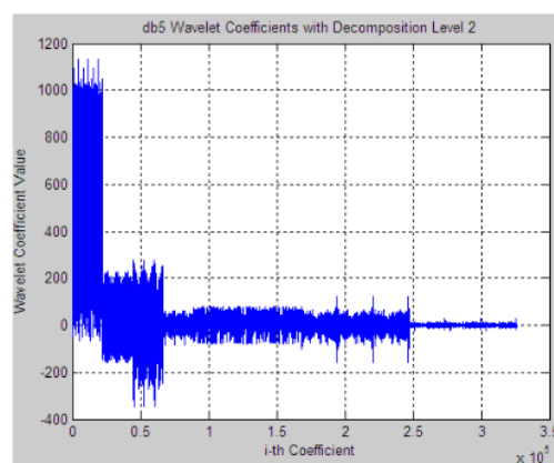
Figure 4. Wavelet coefficient values for db5, decomposition level 2.
