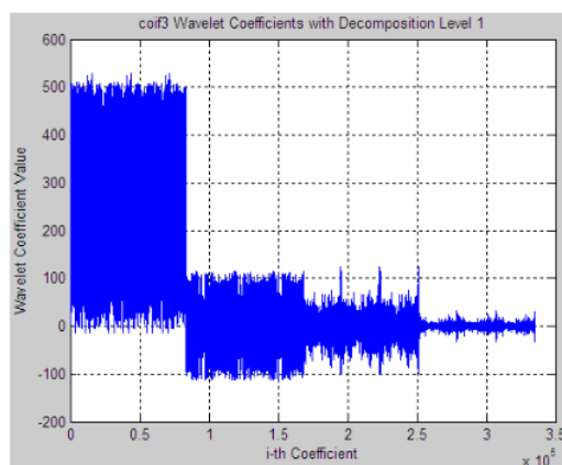
Figure 5. Wavelet coefficient values for coif3, decomposition level 1.
