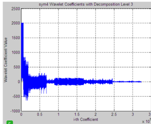
Figure 6. Wavelet coefficient values for sym4, decomposition level 3.
