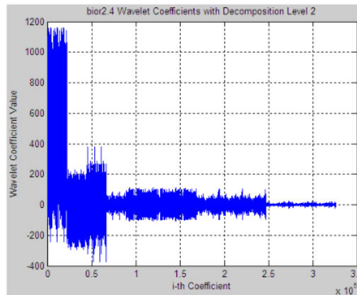
Figure 7. Wavelet coefficient values for bior2.4, decomposition level 2.
