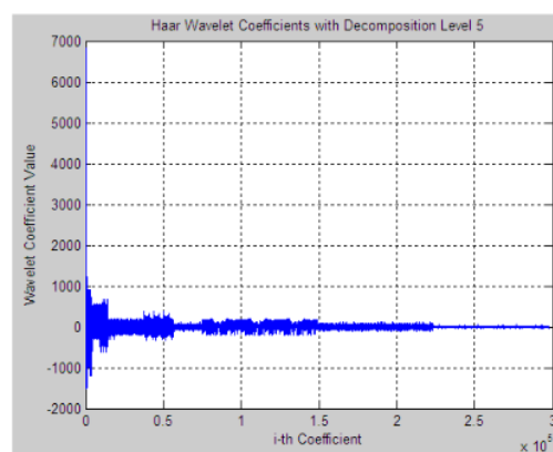
Figure 3. Wavelet coefficient values for Haar, decomposition level 5.
