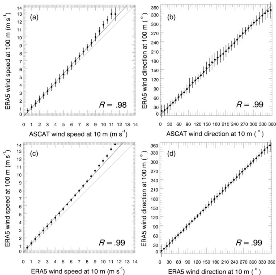
FIGURE 4 Binned scatterplots of (a,c) wind speeds and (b,d) wind directions between 10 m and 100 m. In (a,b), speed and direction between ASCAT and ERA5 are compared, and in (c,d), ERA5 10 m and 100 m wind data are compared. The dots are the means within each bin, and the error bars (vertical lines) are the plus or minus one standard deviation within each bin. The data are extracted from the monthly means of wind vectors from January to December covering the Indonesian seas ( 14^{\circ}\text{S} – 12^{\circ}\text{N} , 92^{\circ} – 150^{\circ}\text{E} ) at a grid interval of 0.25^{\circ} by excluding the data at land grid points. The thick line is the regression line, and R is the correlation coefficient. The ERA5 data plotted in this figure have the same time as ASCAT (number of samples is 219,732). The root mean square errors in (a–d) are the following: 0.55 \text{ m s}^{-1} , 15.5^{\circ} , 0.58 \text{ m s}^{-1} , and 9.66^{\circ} , respectively. The biases in (a–d) are 0.25 \text{ m s}^{-1} , 0.34^{\circ} , 0.44 \text{ m s}^{-1} , and 0.06^{\circ} , respectively
