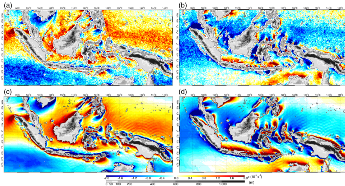
FIGURE 5 Monthly means of wind curl from (a,b) ASCAT and (c,d) hourly data of ERA5 at 10 m in (a,c) January and in (b,d) August [Colour figure can be viewed at wileyonlinelibrary.com ]
