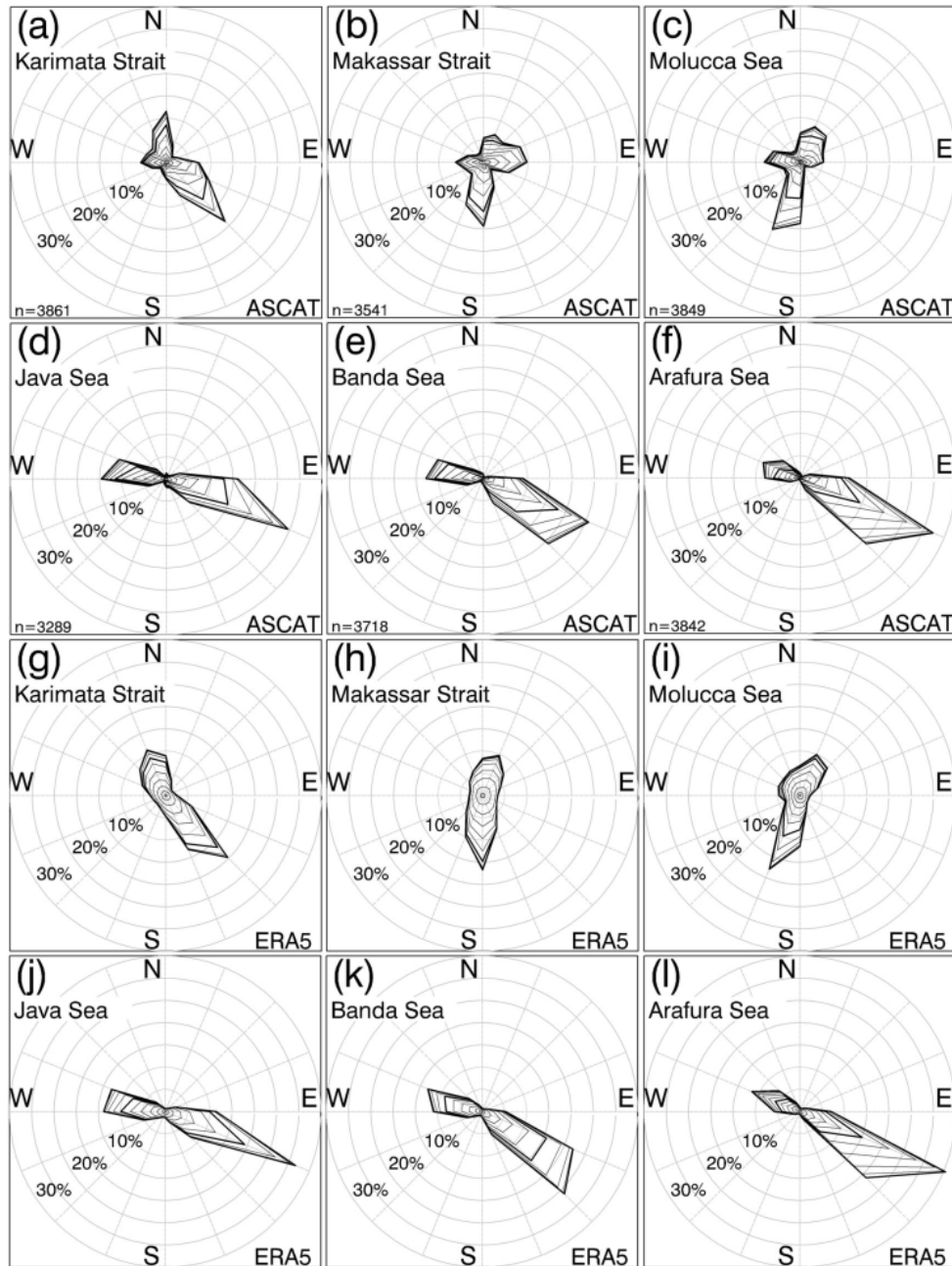
FIGURE 38 Annual wind roses composed of (a–f) ASCAT and (g–l) ERA5 hourly data at 10 m in the selected six locations shown in Figure 1b. Wind direction is defined as the direction from which the wind blows. The compass is divided into 16 sectors. The polygons show the cumulative relative frequency of wind direction with speeds less than a threshold speed for every 1 m s -1 (thin and bold contours). The bold polygons inside are composed of the data with speeds less than 7 m s -1 and the bold outermost polygons are composed of all the data. The circles are the isolines of the cumulative relative frequency of wind direction in the range from 5 to 35%. The numbers of ASCAT samples ( n ) are shown on the bottom left side of each figure. The number of ERA5 data is 78,888 data for each figure
