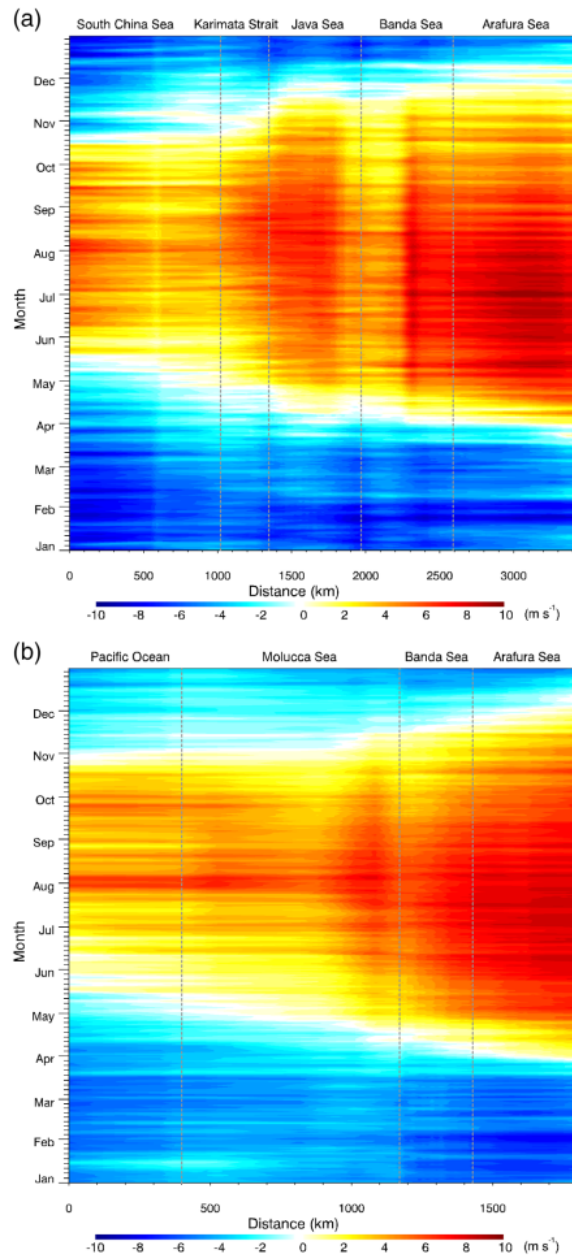
FIGURE 10 Distance-time diagrams of the daily mean of the major-axis wind component along the main monsoon routes denoted by the dashed grey lines in Figure 1b. The ERA5 hourly data at 10 m were used. The defined routes extend to the Arafura Sea from (a) the South China Sea and (b) the Pacific Ocean. Along these routes, the data are sampled at every 0.25^\circ in longitude or latitude and the numbers of sampling locations along the routes are 137 grid points in (a) and 53 grid points in (b). Positive and negative values show the winds blowing during the Australian winter monsoon and the East Asian winter monsoon periods, respectively. The vertical dashed line serves as the only guide of sea boundaries [Colour figure can be viewed at wileyonlinelibrary.com ]
