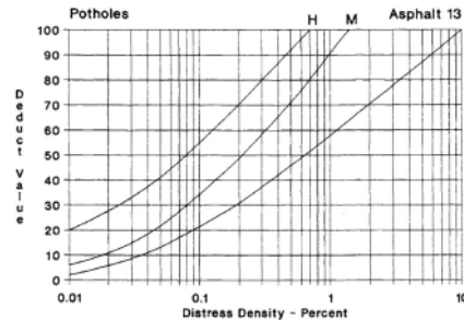
Fig. 1. Deduct value charts for potholes [1, 2]
