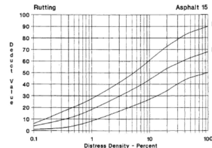
Fig. 2. Deduct value charts for rutting [1, 2]
