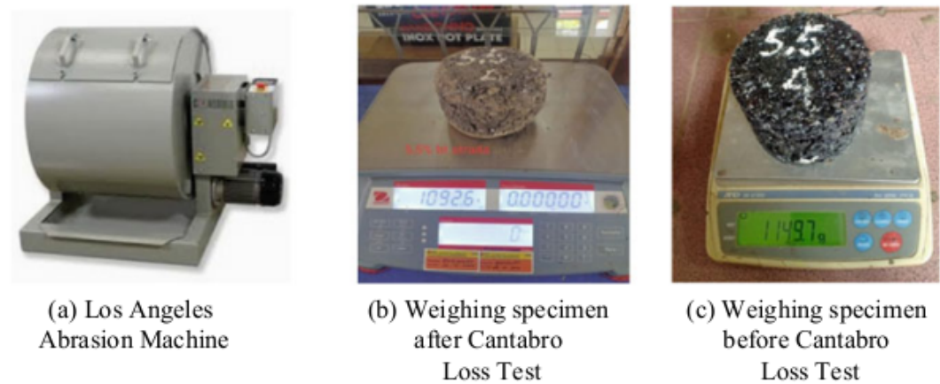
Fig. 2 Cantabro loss test
