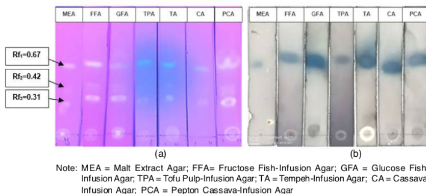
Figure 3. TLC profiles of ethyl acetate extracts of T. longibrachiatum cultivated in various media using n-hexane: ethylacetate (4:1) as mobile phase and their chromatogram spot visualization (a) UV 365 nm, (b) 2 % vanillin- \text{H}_2\text{SO}_4
