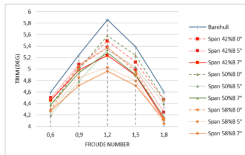
Figure 13. Trim angle comparison
