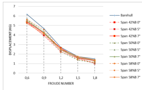
Figure 12. Displacement comparison
