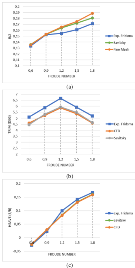
Figure 7. Validation results for resistance, heave, and trim
