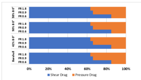
Figure 11. Total drag components
