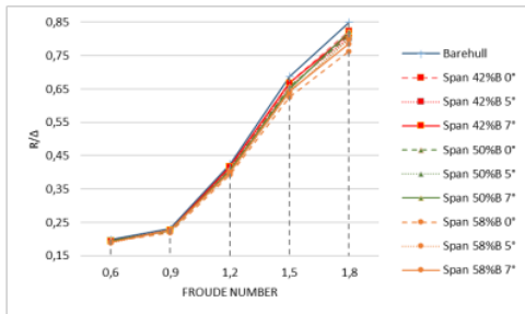
Figure 9. Shear drag comparison
