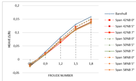
Figure 14. Heave comparison
