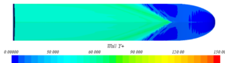
Figure 5. y^+ value at the bottom
