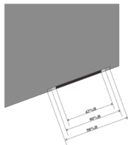
Figure 3. Configuration of stern flap
