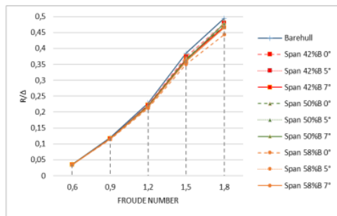
Figure 10. Pressure drag comparison
