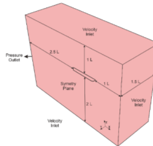
Figure 4. Fluid domain and boundary conditions
