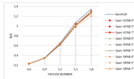
Figure 8. Total drag comparison
