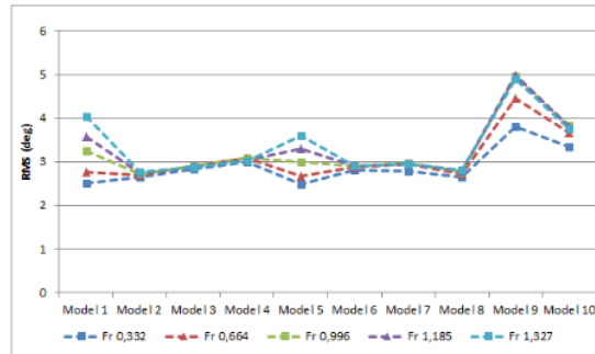
Gambar 9. Grafik RMS Rolling Sea State 3
