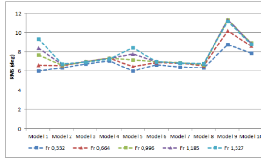
Gambar 11. Grafik RMS Rolling Sea State 5
