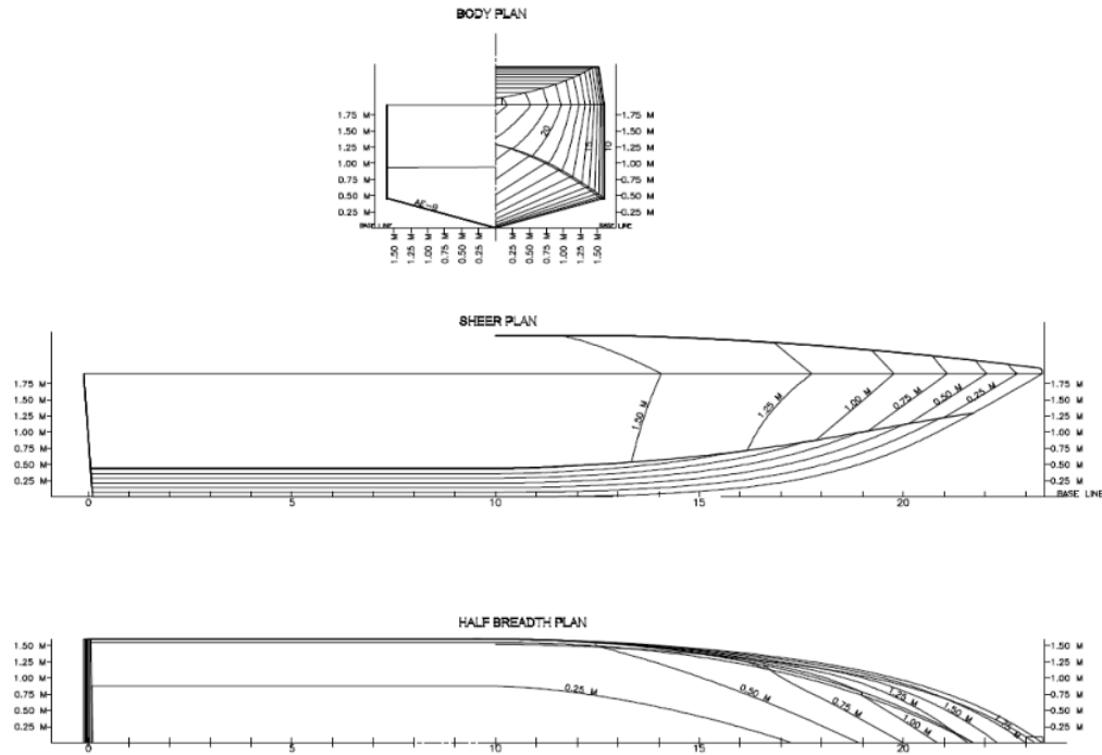
Gambar 2. Geometri 2-D Kapal Patroli
