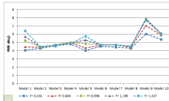
Gambar 10. Grafik RMS Rolling Sea State 4
