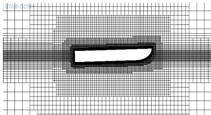
Figure 6. Morphing mesh before deformation
