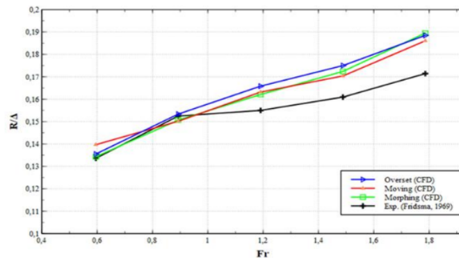
Figure 12. Resistance
