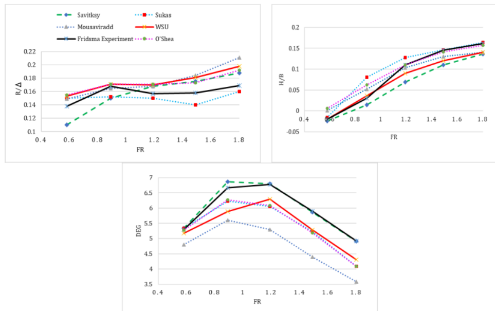
Figure 15. Comparison of drag, trim and heave [23]
