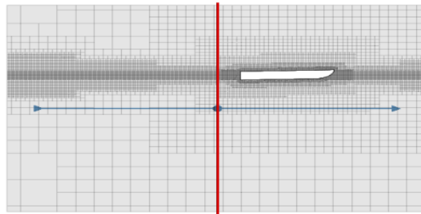
Figure 7. Moving mesh before analyzed
