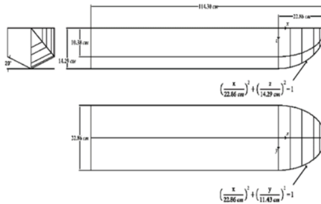
Figure 2. Lines plan of Fridsma hull form
