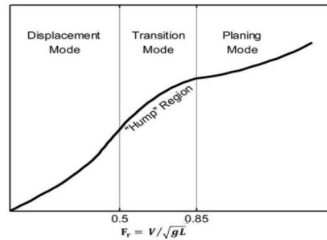
Figure 1. Ship classification based on froude number [14]
