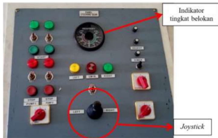
Gambar 4. Panel Steering Gear di Anjungan
