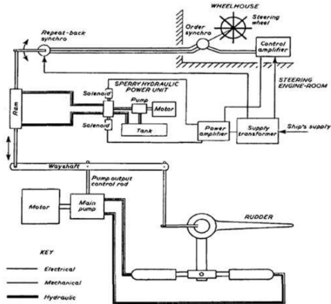
Gambar 1. Diagram Sistem Hydraulic Steering [3]
