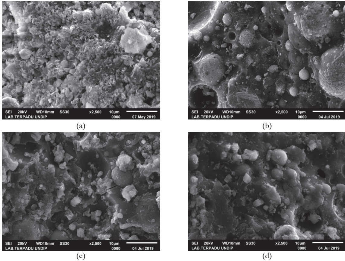
FIGURE 3. SEM micrographs of fly ash-based geopolymer after adsorption of \text{Cu}^{2+} (a), \text{Fe}^{2+} (b), \text{Mn}^{2+} (c), and \text{Zn}^{2+} (d) ions.
