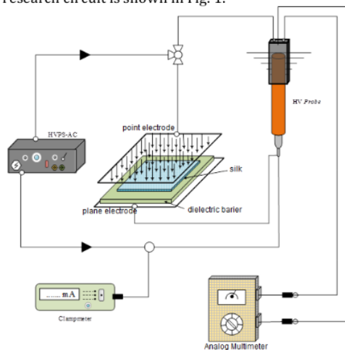
Fig.1: Scheme of the research instrument.
