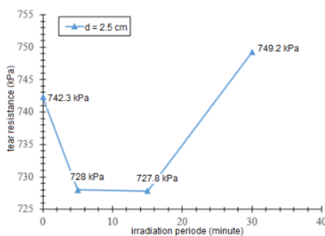
Fig. 6: Relationship between tear resistance (kPa) and irradiation period (minute) of the natural silk.
