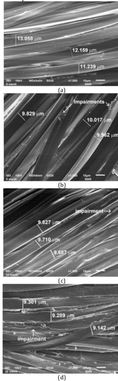
Fig. 4: Results of SEM image on natural silk; (a) non-irradiated, (b) irradiated for 5 minutes, (c) irradiated for 15 minutes, (d) irradiated for 30 minutes.
