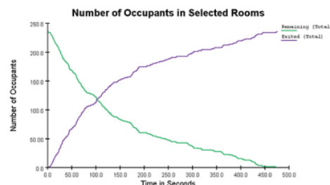
Figure 3. Evacuation Simulation Results Graph
