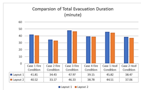
Figure 12. Comparison Chart of Total Evacuation Duration
