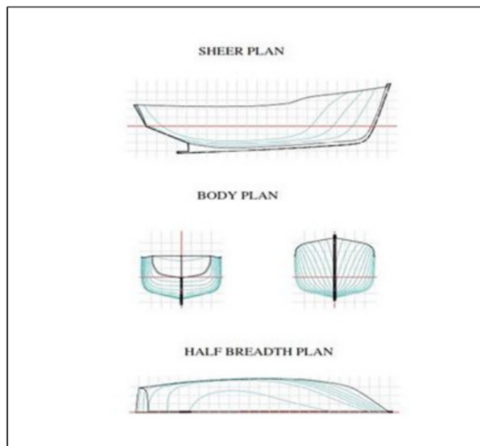
Figure 2. Redrawing of Batang Type Traditional Fishing Boat
