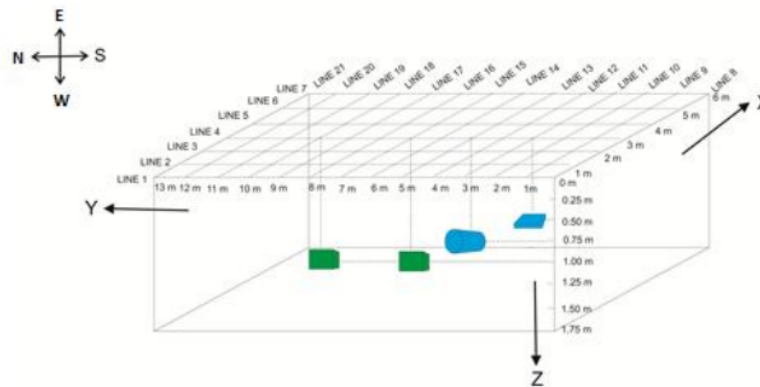
Figure 3 Model scale survey design
