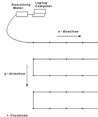
Figure 1 Preparation of grid electrodes for 3-dimensional survey[11].
