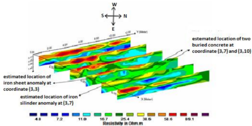
Figure 6. Vertical cross section (y-z) arranged horizontally
