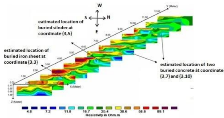
Figure 5 Vertical cross section (x-z) arranged horizontally
