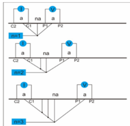
Figure 2 Dipole-Dipole Configuration[12]
