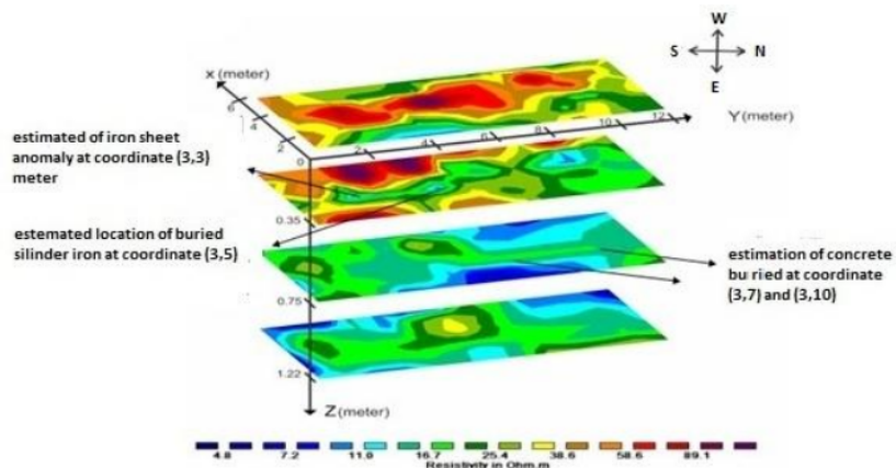
Figure 4 Horizontal cross section (x-y) arranged vertically
