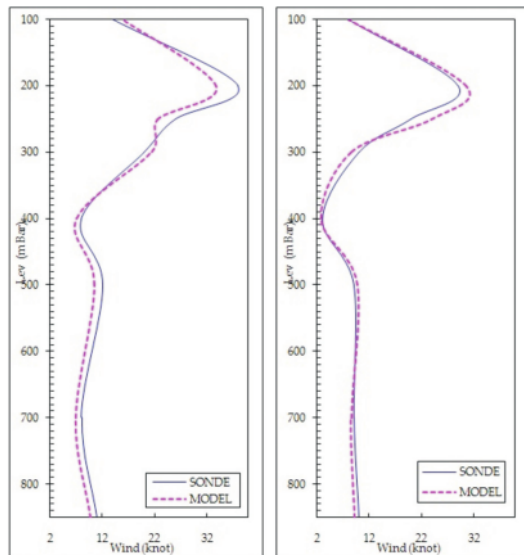
Fig. 4. Wind Speed data validation on October 24 2017 12 UTC and October 24, 2017, 00 UTC Batik Air ID6890
