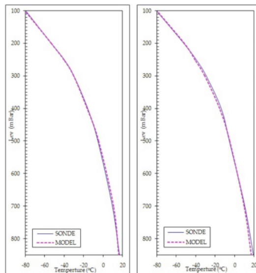
Fig. 5. Temperature data validation on October 24 2017 12 UTC and October 24, 2017, 00 UTC Batik Air ID6890
