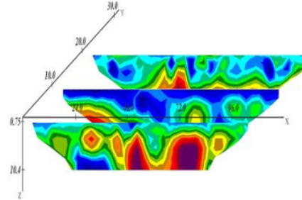
Figure 2 Correlation Field B
