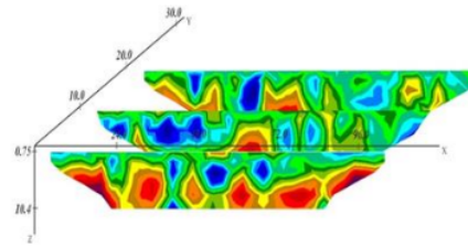
Figure 1 Correlation Field A
