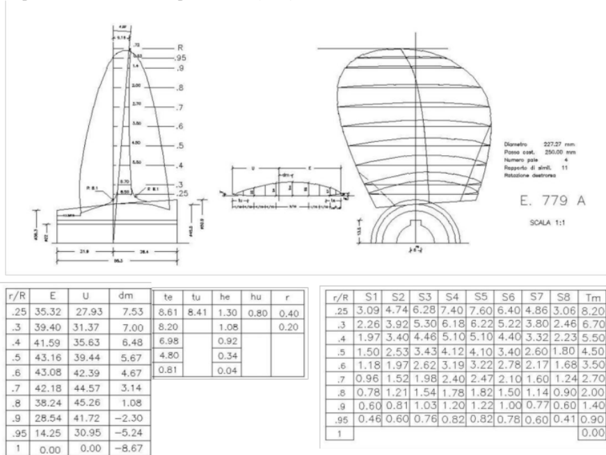
Figure 1. Propeller geometry of INSEAN e779a
