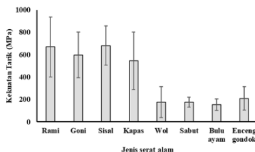
Gambar 1. Kekuatan Tarik Beberapa Serat Alam (Pickering dkk. , 2016; Tumolva, 2013; Bordoloi dkk. , 2018; Chonsakorn dkk. , 2018; Gashti, 2013; Dittenber dan Ganga Rao, 2011; Cheng dkk. , 2009).
