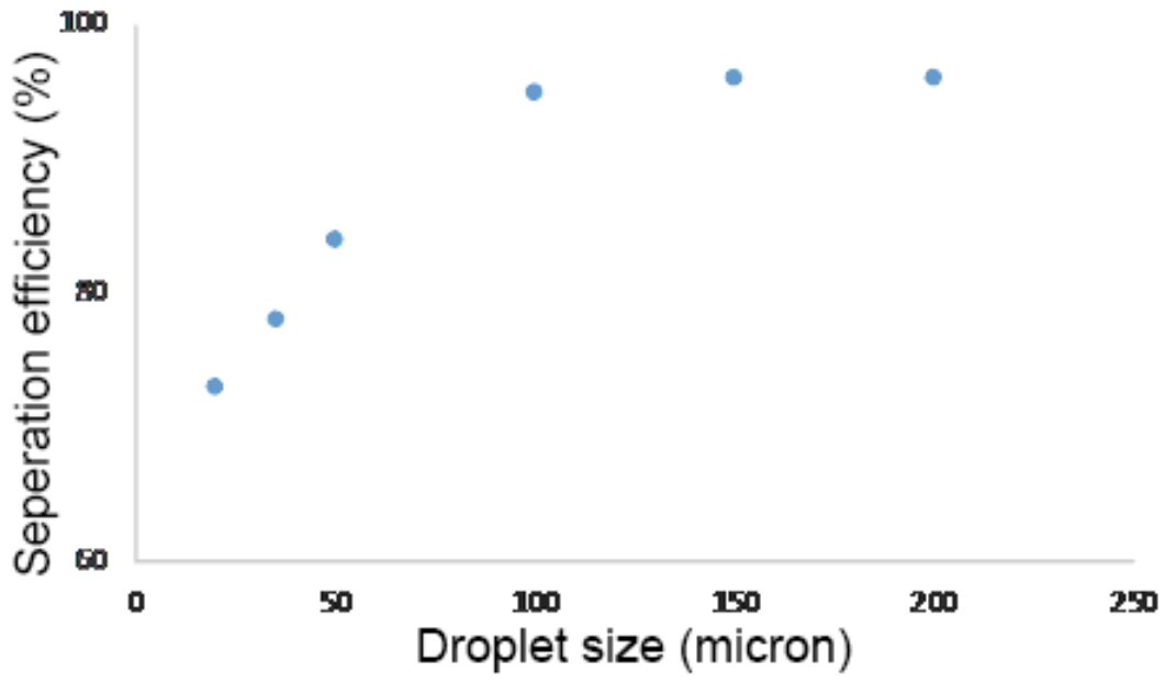
Fig. 9- Effect of droplet size on the separation efficiency.
