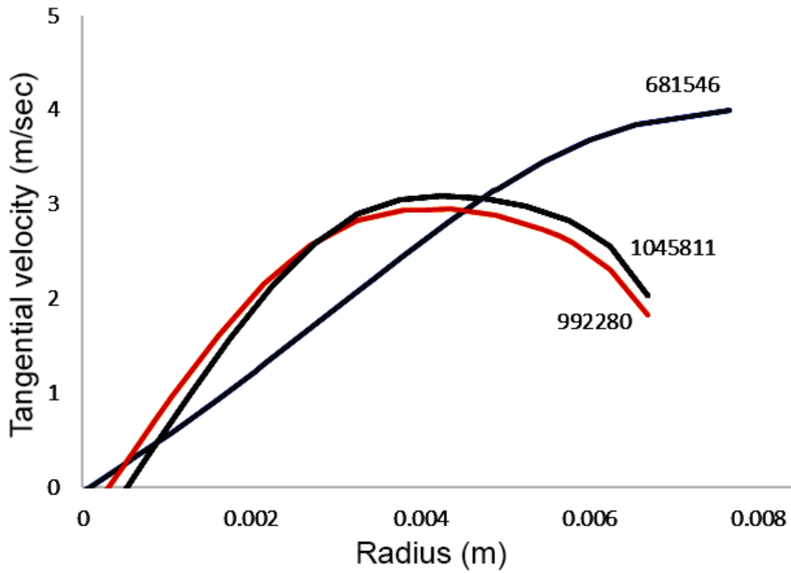
Fig. 4- Calculation of tangential velocity versus radiuses if the hydrocyclone with different calculation meshes.
