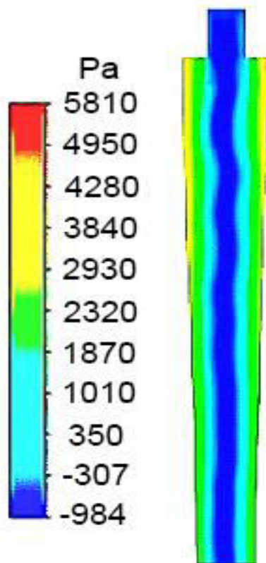
Fig. 7- a) Static pressure diagram and b) contour, within the hydrocyclone.
