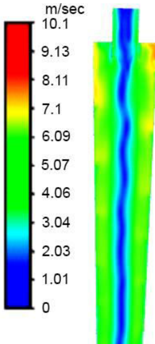
Fig. 8- a) Diagram and b) contour of velocity magnitude within the hydrocyclone.
