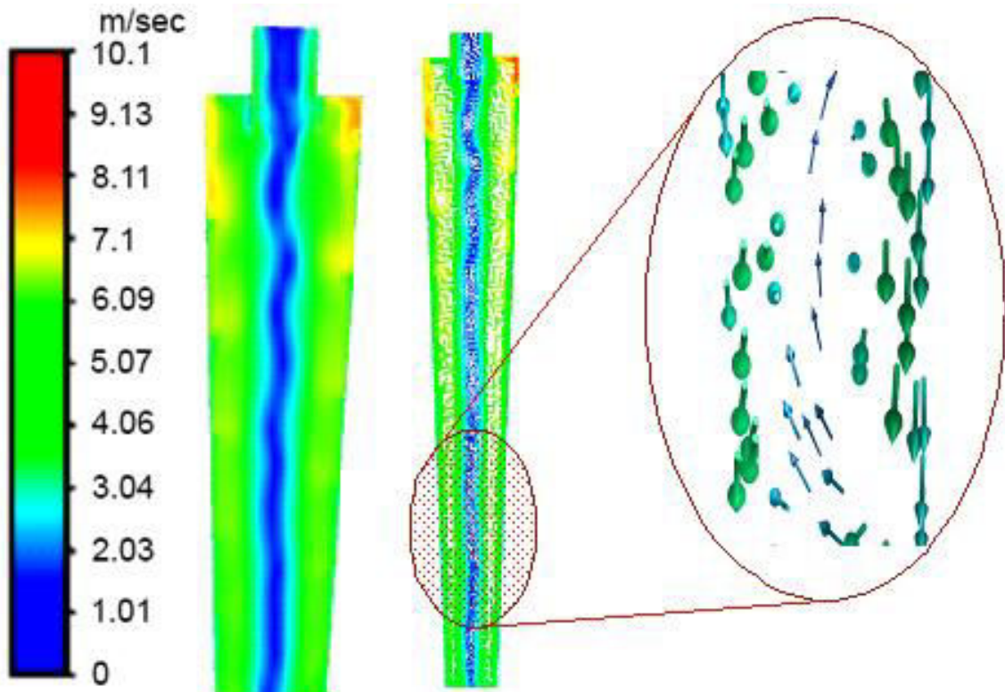
Fig. 10- The fluid flows vectors inside the hydrocyclone.
