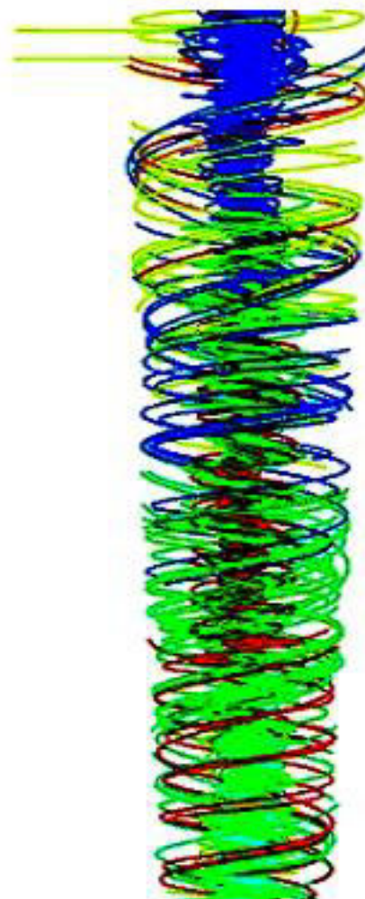
Fig. 6- Streamlines of the continuous phase (water).
