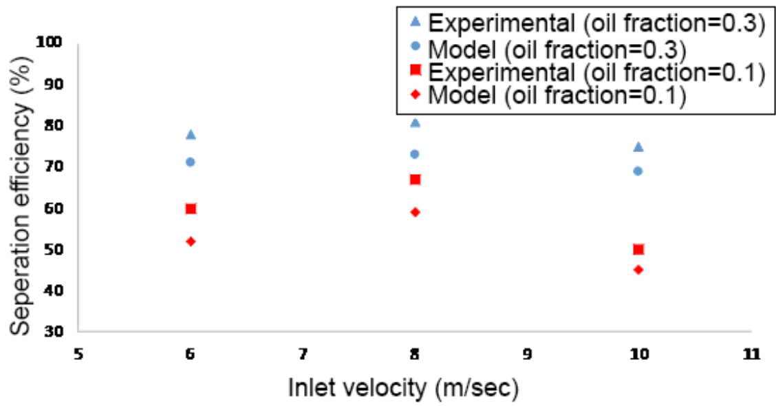
Fig. 5- Comparison of simulation results with experimental data [42].
