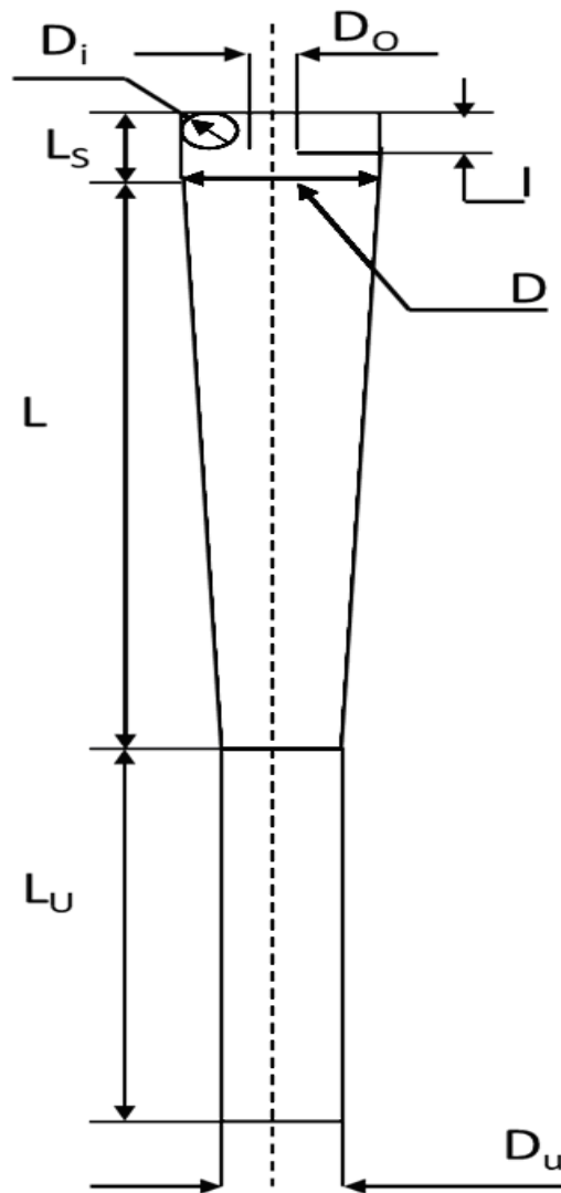
Fig 2- Hydrocyclon geometry.
