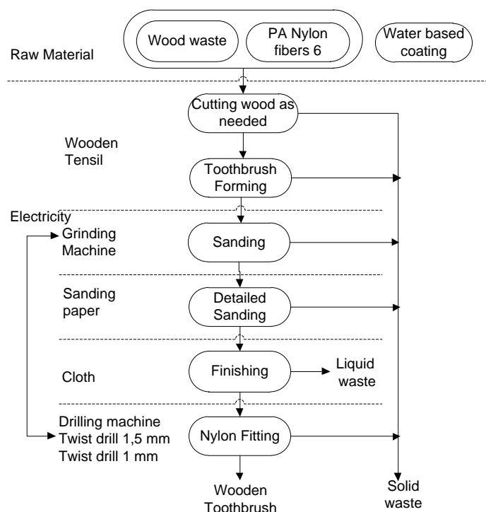
Figure 7. The production process flow of a wood waste toothbrush
