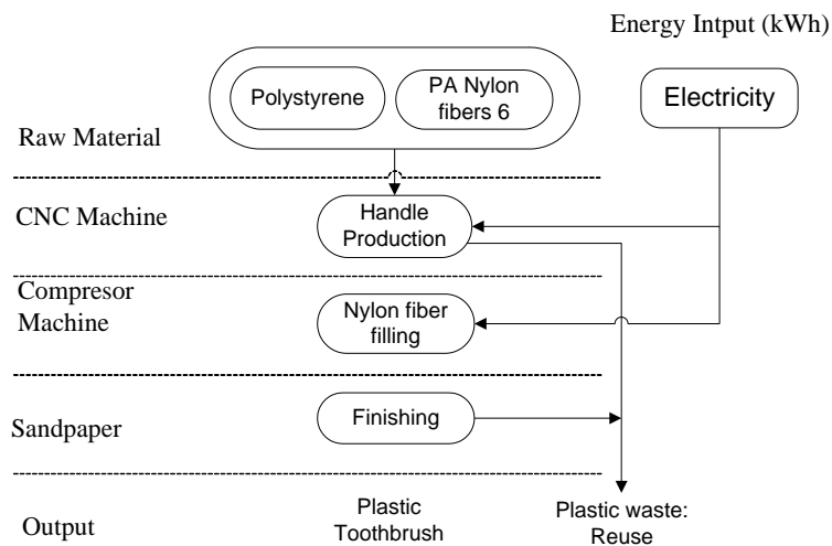
Figure 6. Process production of polystyrene toothbrush
